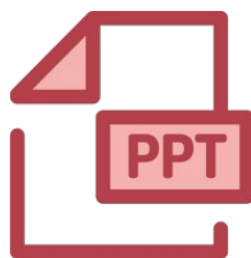
Presentation Software
